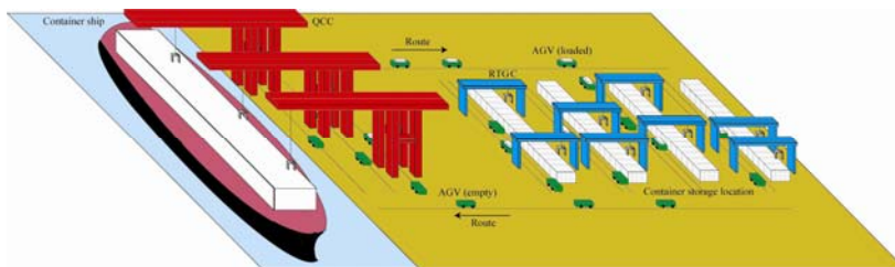
Fig. 1 The Horizontal -type AGV Transportation System in Automated Container Terminal
