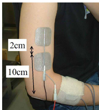
Fig. 2 Electrical Stimulation Electrodes
