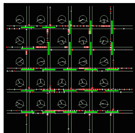
Fig. 2 Traffic Simulator
